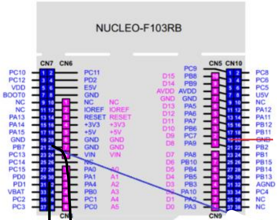
Figure 14. NUCLEO-F103RB
