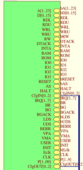
Slot Slot.sch
