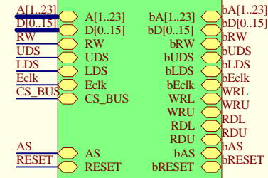
Buformagistrali Bufor.sch
