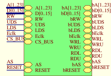
Buformagistrali Bufor.sch
